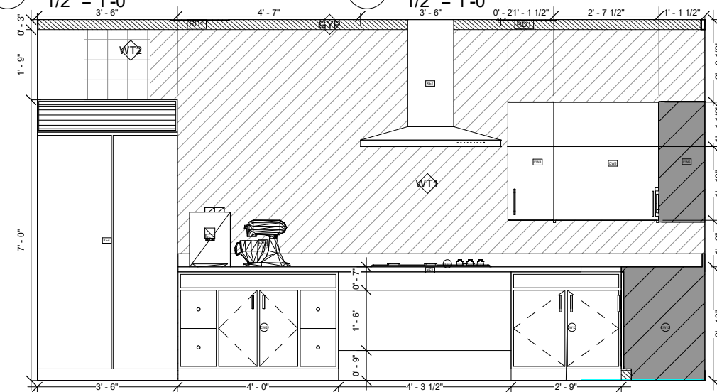
2 KITCHEN ELEVATION2 1 KITCHEN ELEVATION1
